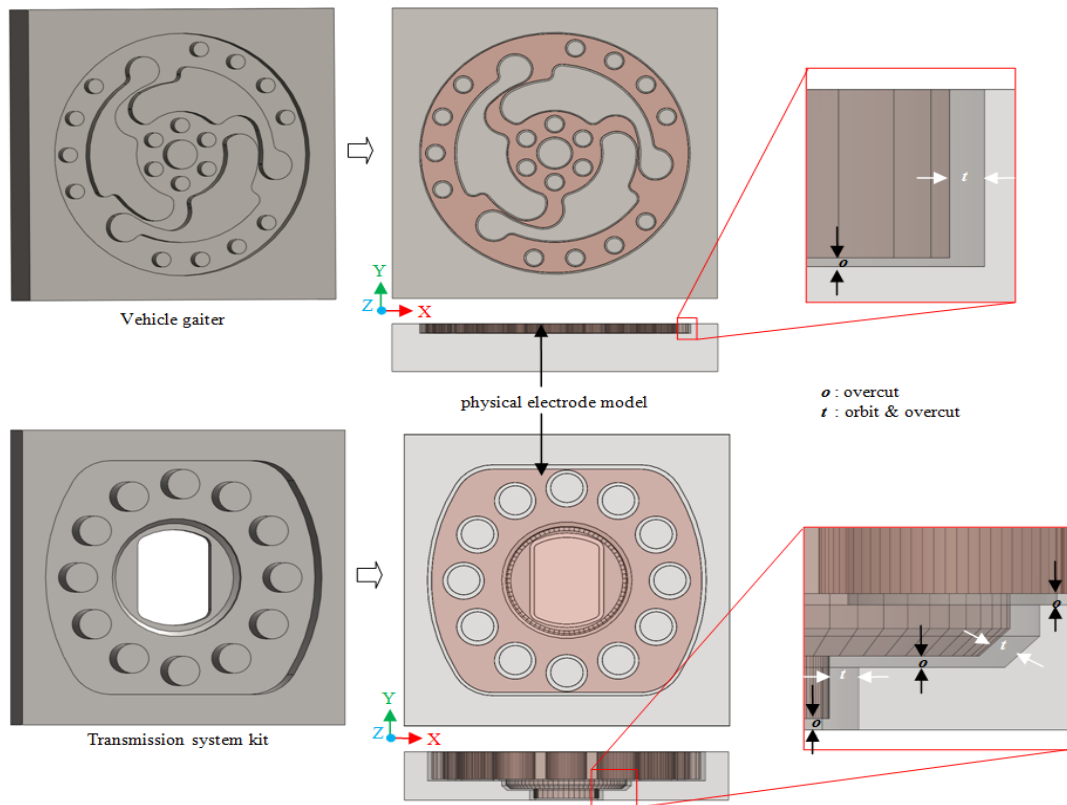
Figure 9. Electrode design for automotive parts
