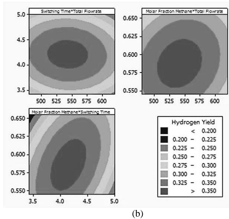
Figure 5. (a) Contour plots for methane conversion (b) Contour plots of hydrogen yield
