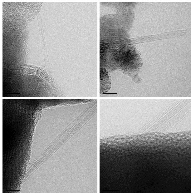
Figure 7. TEM images of individual SWNTs
