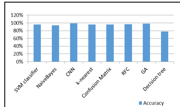
Figure 2: Comparison Accuracy Chart
