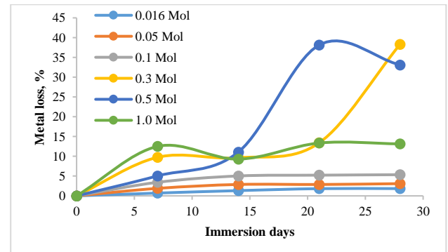
Figure 6 Corrosion rate for ungalvanised cold-formed steel coupons in \text{CuSO}_4
