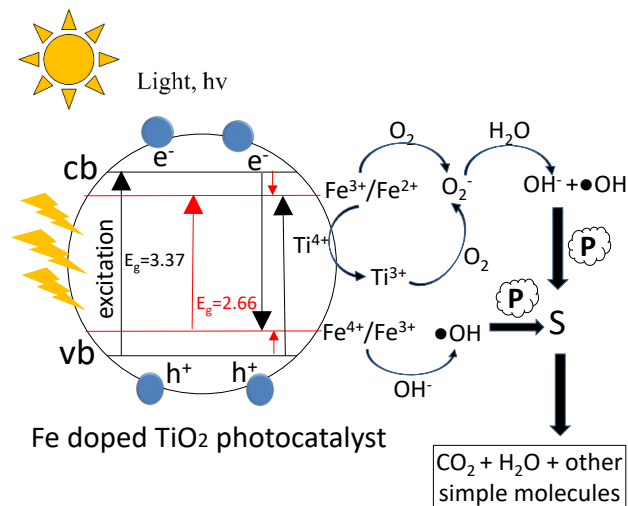
Figure 11 The proposed schematic mechanism diagram of photocatalytic reaction occurs on the Fe. doped TiO_2 surface
