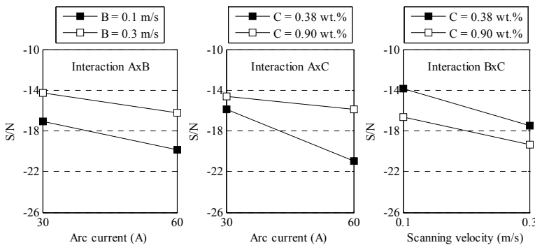
Figure 7 Interaction graphs for all processing parameters on hardened depth
