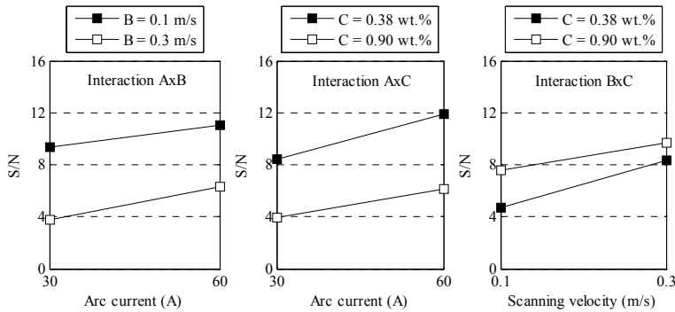
Figure 8 Interaction graphs for all processing parameters on surface roughness
