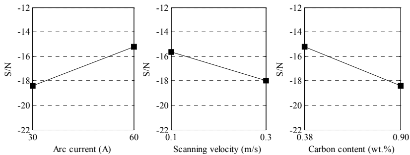
Figure 5 S/N response graphs for all processing parameters on hardened depth
