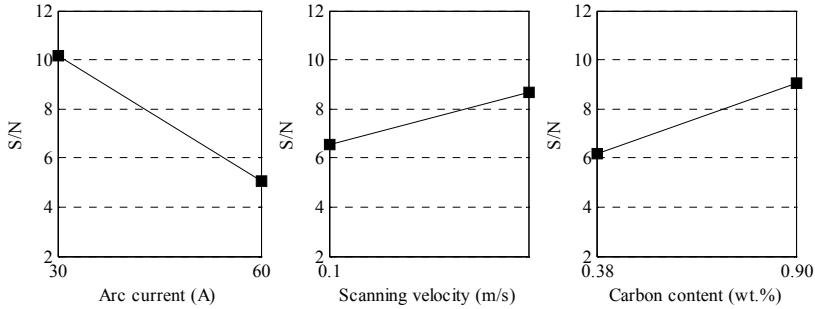
Figure 6 S/N response graphs for all processing parameters on surface roughness
