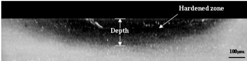
Figure 2 Schematic of hardened zone cross section
