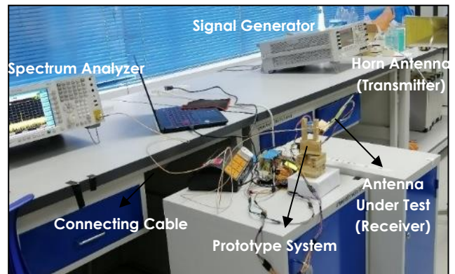
Figure 8 Setup of Signal Strength of Antenna Measurement
