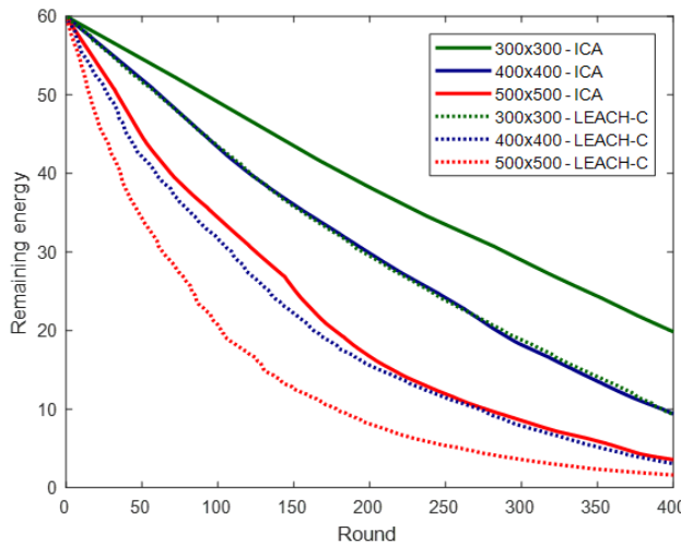
Figure 10 Remaining energy per round for different size of network
