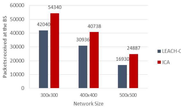
Figure 9 Packets receive at the base station for different size of network area
