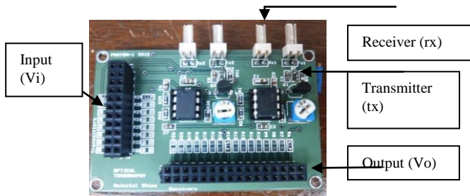
Figure 3 Circuit controlling two transmitters and two receivers on one PCB
