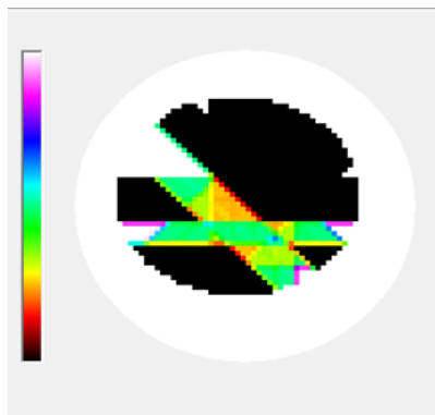
Figure 8 Air gap in the liquid phase
