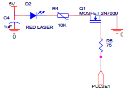
Figure 2 Transmitter circuit
