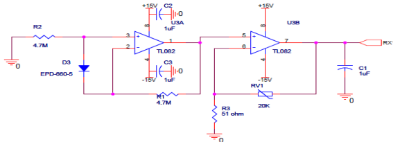
Figure 1 Receiver circuit
