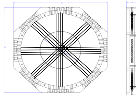
Figure 7 Top view of the jig with sensors
