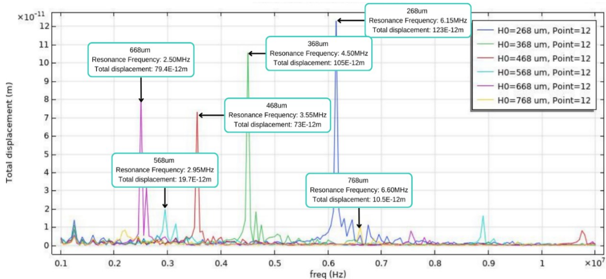
Figure 2 Graph plotted for varying quartz thickness simulation by COMSOL Multiphysics software
