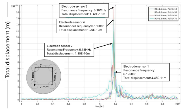
Figure 14 Simulation outcome for 4-channel QCM with 7 mm c2c distance
