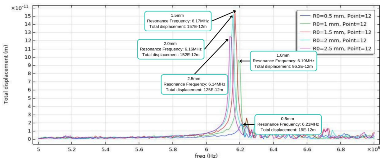
Figure 3 Graph plotted for varying radius of electrode sensor simulation by COMSOL Multiphysics software
