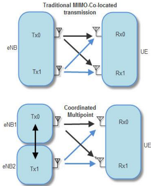
Figure 3 The differences between traditional MIMO and CoMP
