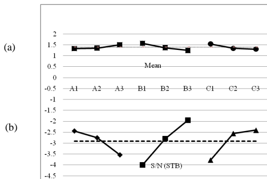
Figure 2 Control factor’s response plot (a) Mean (mm), (b) Signal Noise ratio (dB)
