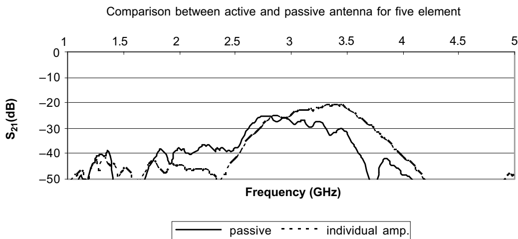
Figure 13 S_{21} response relative to passive
