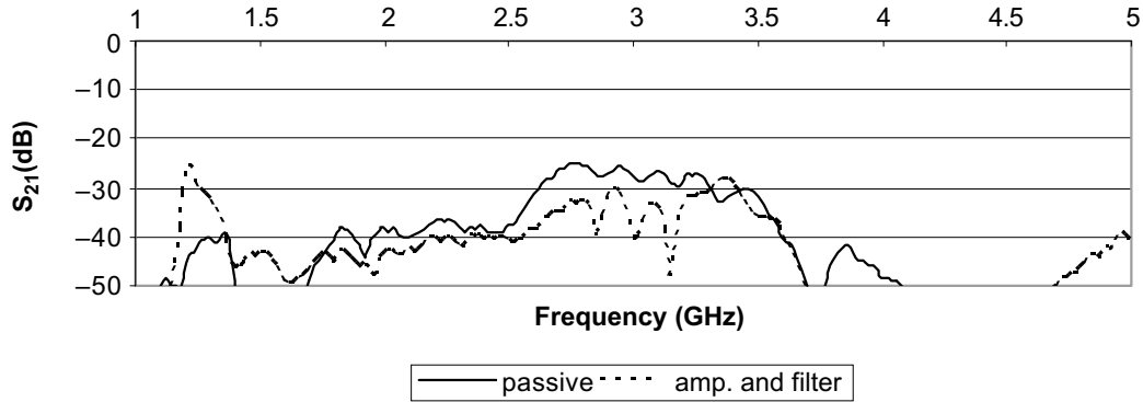
Figure 16 S_{21} response relative to passive
