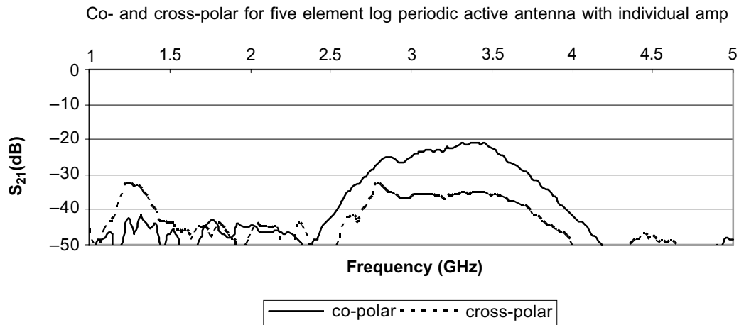
Figure 12 Cross polar isolation
