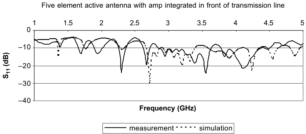
Figure 5 Input return loss
