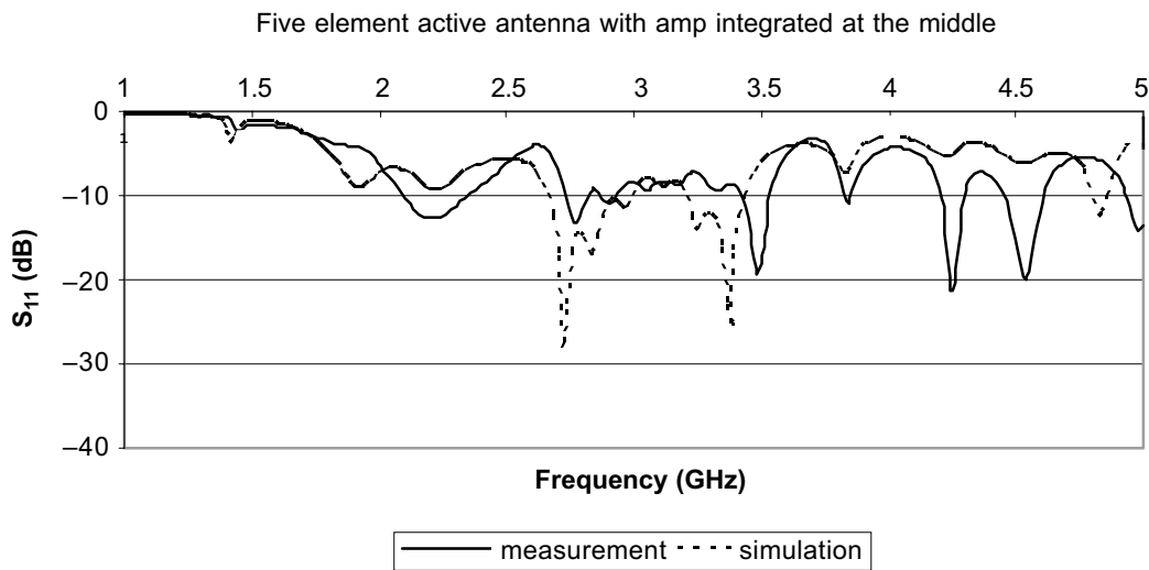
Figure 8 Input return loss
