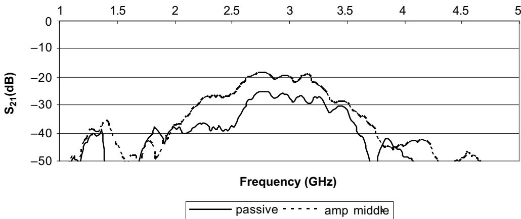
Figure 10 S_{21} response relative to passive
