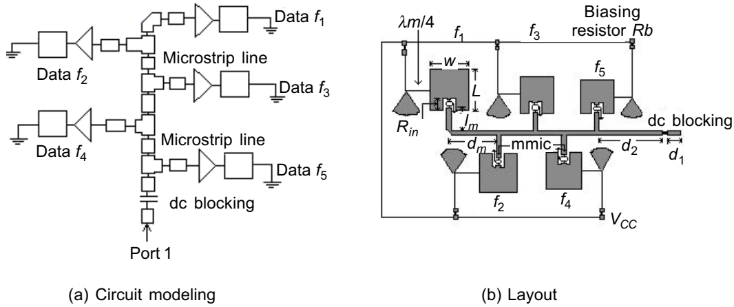
Figure 3 Circuit modeling and layout of amplifier integration into each element of LPA
