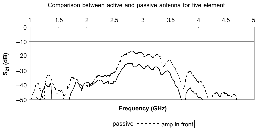
Figure 7 S_{21} response relative to passive LPA
