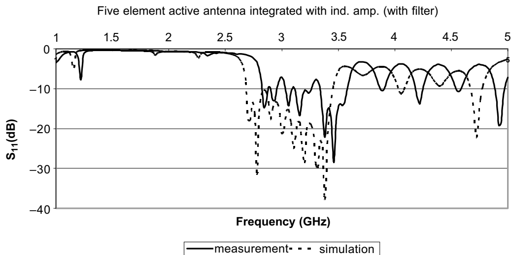
Figure 14 Input return loss
