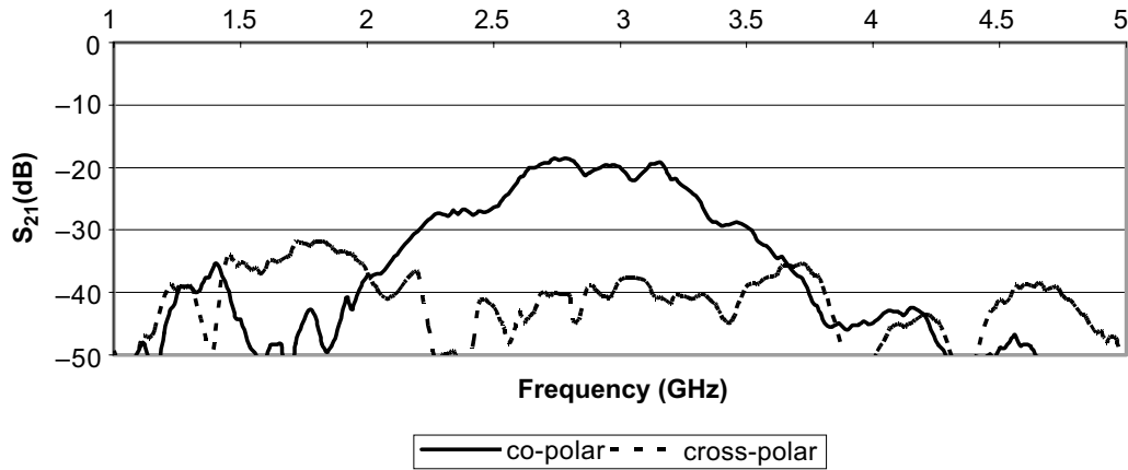
Figure 9 Co- and cross-polar isolation
