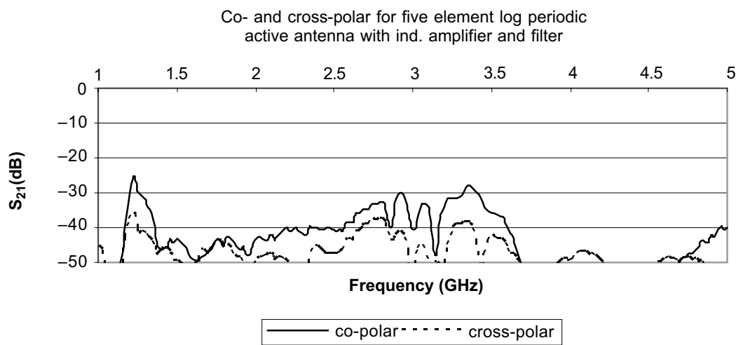
Figure 15 Co- and cross-polar isolation
