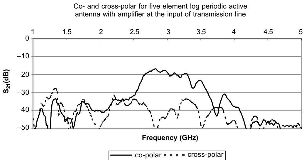
Figure 6 S_{21} response for active LPA
