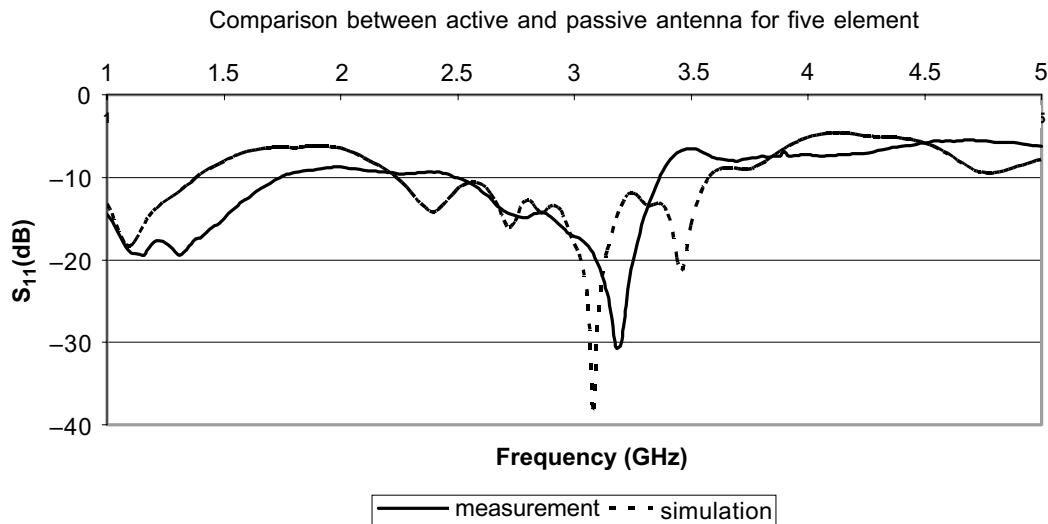
Figure 11 Input return loss
