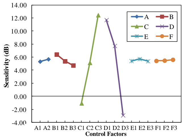
Figure 6 Factor effect plot for Sensitivity
