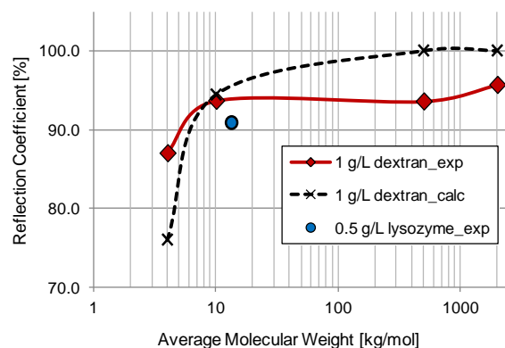
Figure 3 The comparison between experimental (solid line) and calculated data (dashed-line) of the reflection coefficient of test solutes: (i) dextran from various molecular weights, and (ii) lysozyme, in M15DC05 gel
