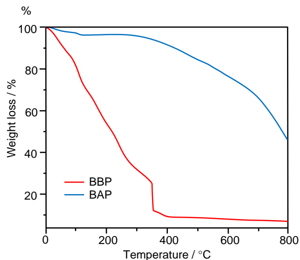
Figure 4 Thermogravimetric analysis curves of freeze-dried bilimbi (BBP) and pyrolysed bilimbi (BAP)
