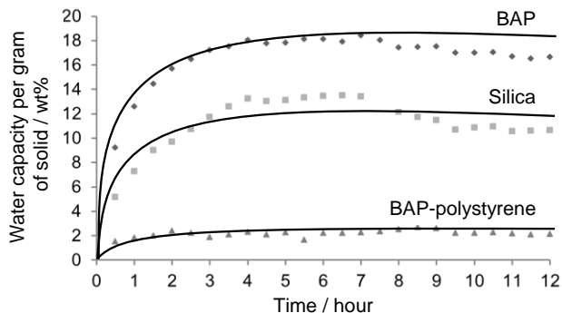
Figure 5 The percentage of water adsorption on the surface of pyrolysed bilimbi (BAP), bilimbi after pyrolysis covered with polystyrene (BAP-polystyrene) and silica
