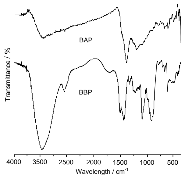
Figure 3 FTIR spectra of pyrolysed bilimbi (BAP) and freeze-dried bilimbi (BBP)
