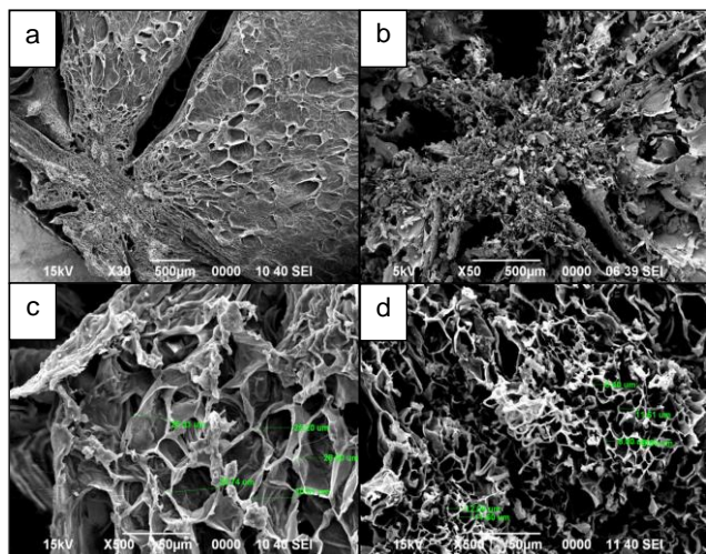
Figure 2 SEM images of (a) freeze-dried bilimbi, (b) bilimbi after pyrolysis, (c) pore structure of bilimbi after pyrolysis at the outer part and (d) pore structure of bilimbi after pyrolysis at the center
