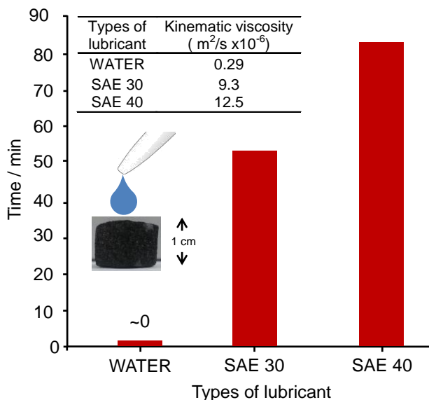
Figure 6 The kinematic diffusion of different types of lubricant through pyrolysed bilimbi (BAP)
