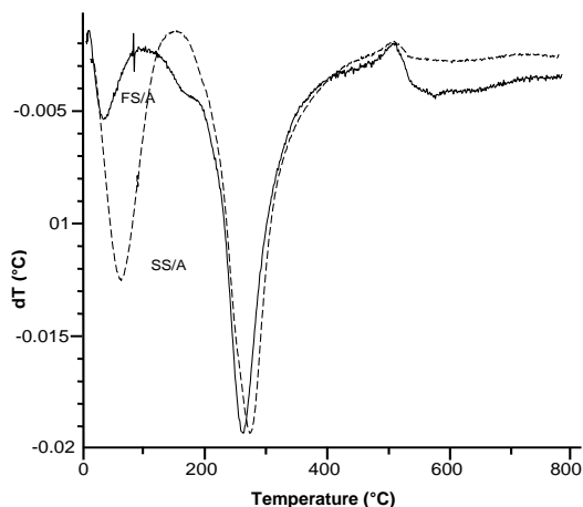
Figure 5 Differential thermal analysis of SS/A and FS/A
