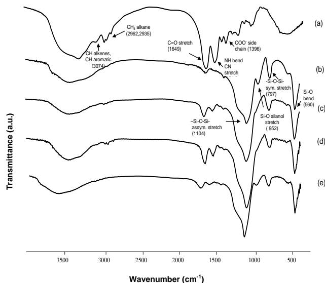
Figure 3 FTIR spectra of obtained samples (a) albumin (b) silica (c) FS/A (d) FS/A-N and (e) SS/A
