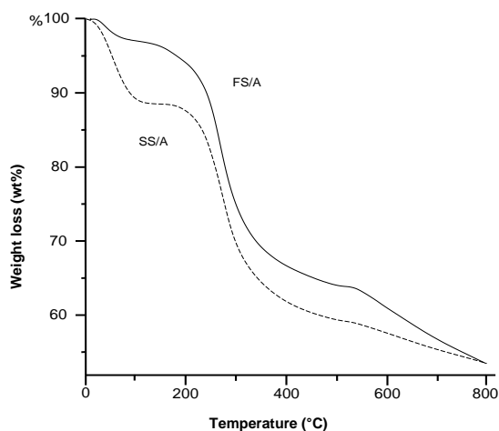
Figure 4 Thermogravimetric curves of SS/A and FS/A
