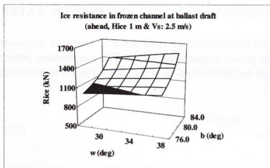
Figure 10 Ice resistance in frozen channel at ballast draft, ahead, H-ice: 1.0 m and Vs: 2.5 m/s
