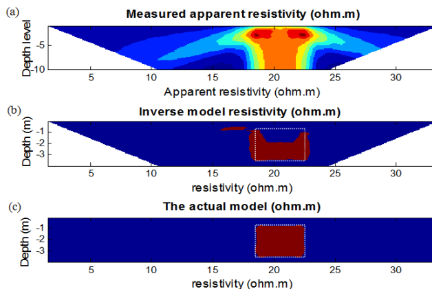
Figure 3 The inversion using synthetic data; (a) Apparent resistivity from the forward model, (b) Inversion result using RBFNN metamodel, (c) The actual test model
