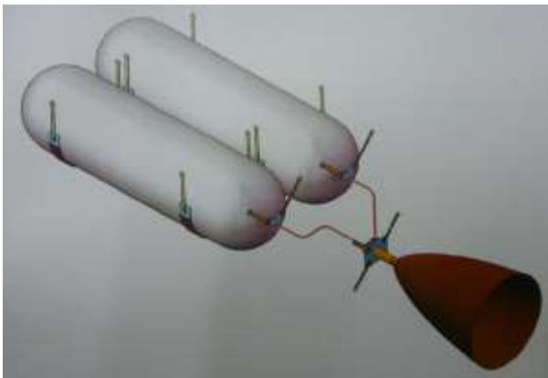
Figure 35 Conceptual design of nitrogen tetroxide/monomethyl hydrazine liquid propellant rocket engine 36
