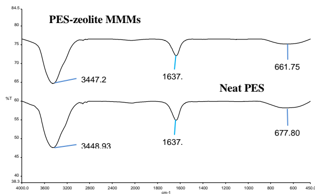
Figure 2 FTIR spectroscopy results for PES-zeolite MMM at zeolite loading 10wt% and neat PES membrane
