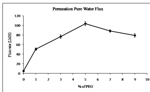
Figure 1 Permeation pure water flux versus percentage (%) of PEG concentration.
