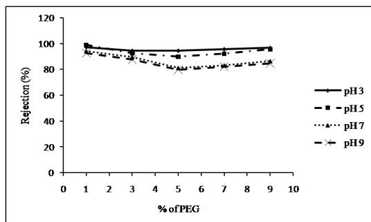
Figure 3 Rejection (%) of BSA using PSf-based membrane
