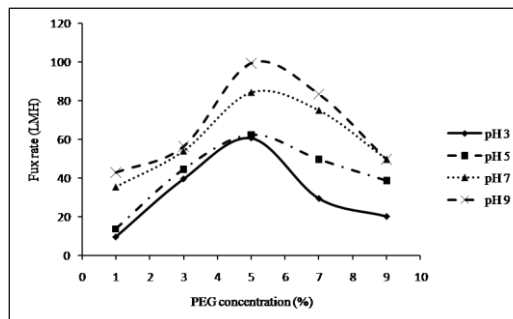
Figure 2 Membrane permeability in rejection of BSA using PSf-based membrane
