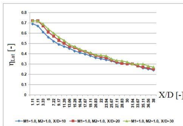
Figure 13 The effect of row spacing on adiabatic film cooling effectiveness [70]
