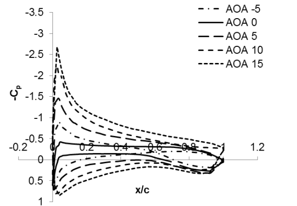
Figure 10 Chordwise surface pressure distribution of the CAC at Mach 0.80
