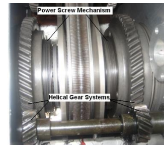
Figure 6 The helical gears and power screw mechanisms
