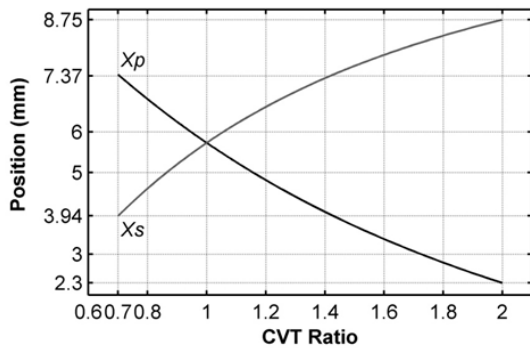
Figure 3 Relationship between pulley positions and CVT ratio
