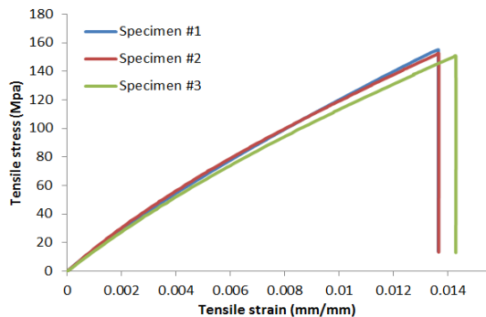
Figure 2 Tensile stress-strain curves of chopped strand mat glass fibre/polyester facesheet material specimens
