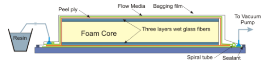
Figure 3 The schematic of vacuum infusion process for foam core sandwich panel
