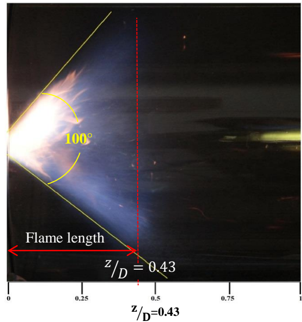
Figure 8 Angle of flame using 60° radial swirler
