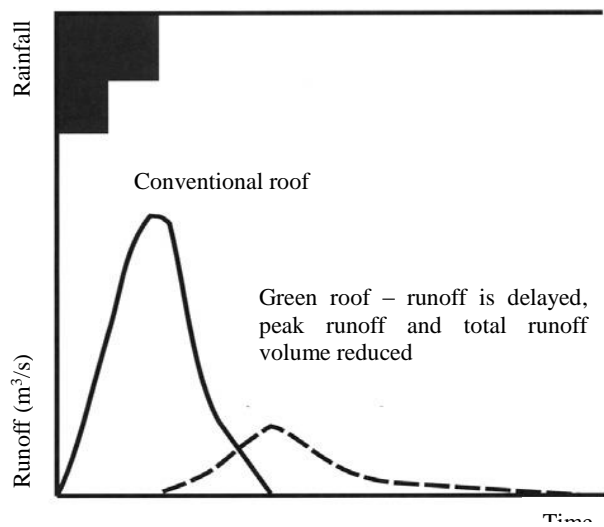
Figure 7 Rainfall runoff response (schematic) [35]
