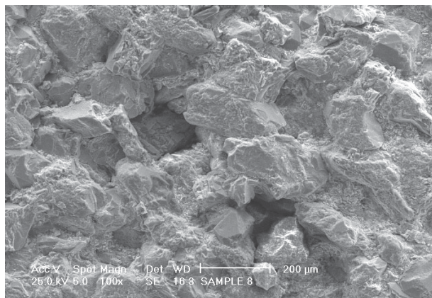
Figure 6 SEM image of a Berea sandstone core sample, damaged at 150 psi (1034.2 kPa) at an angle of 90°
