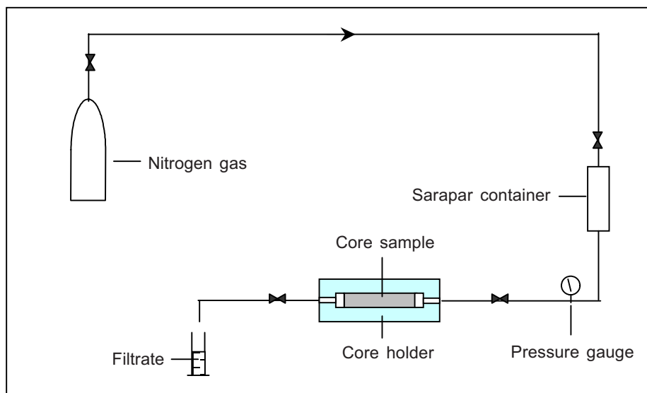
Figure 1 Schematic of the permeability measurement apparatus
