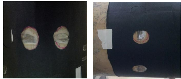
Figure 8 Internal flaws simulated on the pipe surface
