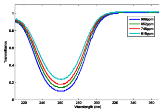
Figure 5 Transmittance measurements for various ozone concentration at range of wavelength from 210 nm to 370 nm.
