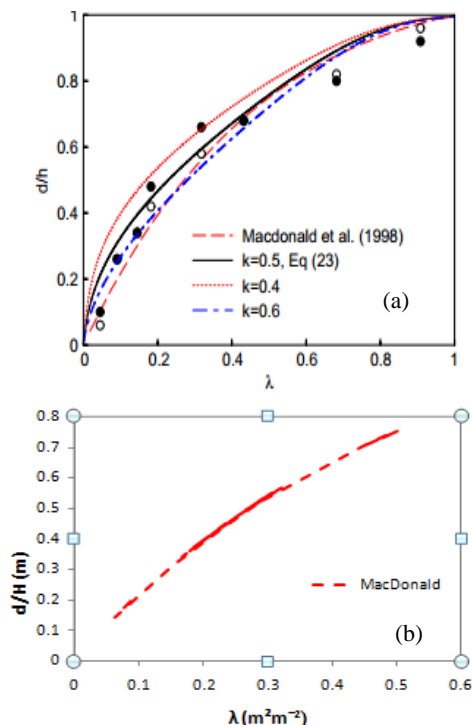
Figure 14 Comparison between d/H values obtained using wind tunnel experiment (a) 24 and values obtained in this study with assumed with direction of 90^\circ (b)
