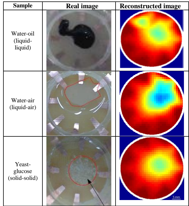
Figure 3 The reconstructed images for different multiphase sample
