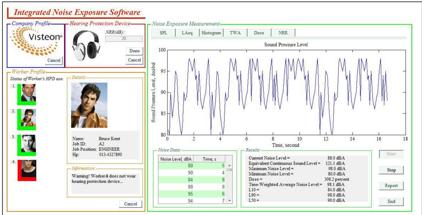
Figure 6 The prototyping model of integrated noise exposure software
