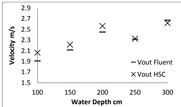
Figure 4 Comparison between CFD and experimental results for the vortex pool system
