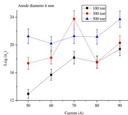
Figure 3 Density of arc plasma for arc current 50 A, 60 A, 70 A, 80 A & 90 A at pressure 100 torr, 300 torr and 500 torr
