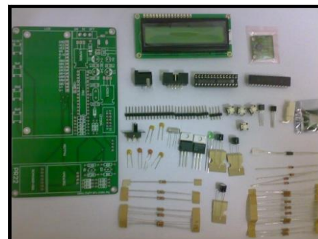
Figure 3(a) PIC board before combining all the components
