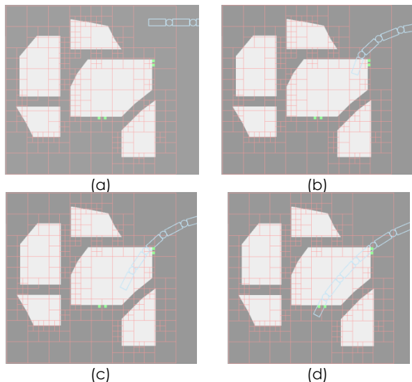
Figure 5 Progress of the algorithm in (a) to (d) sequence. The manipulator (blue rectangle/circle) ignores deformable object (gray) in its path as long as it does not inflict too much pressure to damage it. Red lines shows leaves cells
