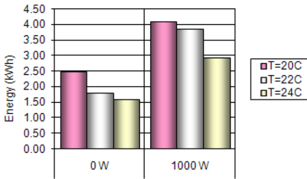
Figure 11 The energy consumption distribution for on/off control
