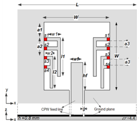
Figure 1 Proposed antenna structure
