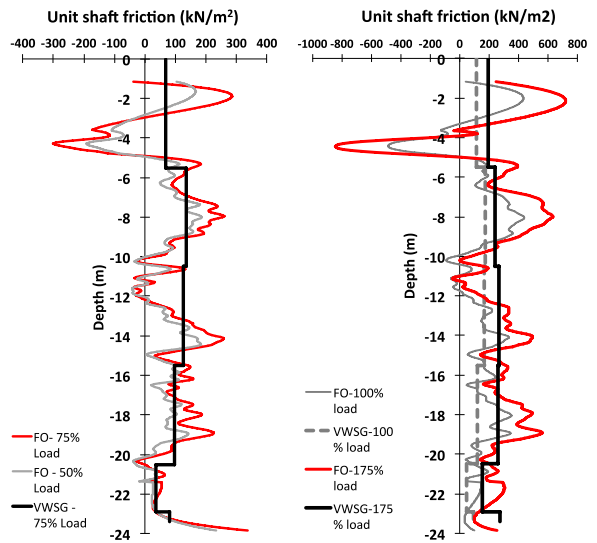
(a) First cycle (b) Second cycle
