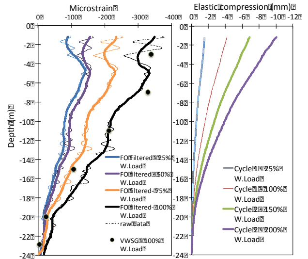
Figure 12 Example of FO filtered data from the first cycle
