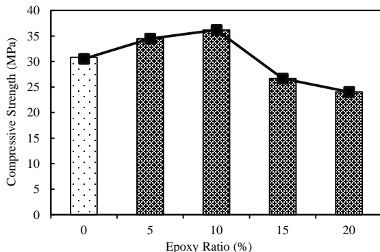
Figure 1 Relationship between compressive strength and epoxy ratio at 28 days in wet-dry curing condition
