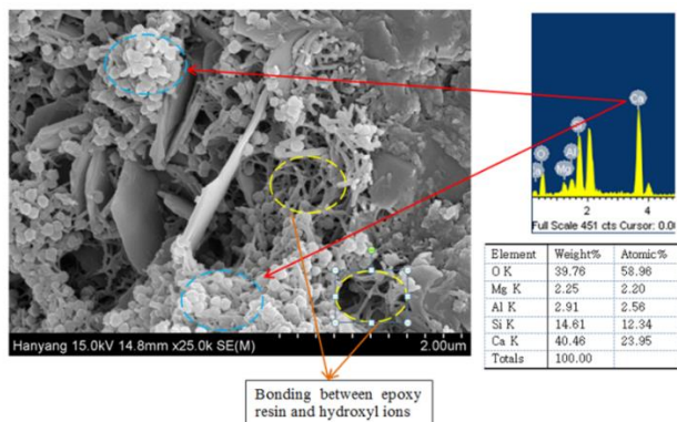
Figure 6 SEM morphology of epoxy-modified mortar
