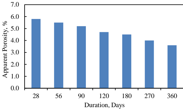
Figure 3 Relationship between porosity of epoxy-modified mortar with curing age
