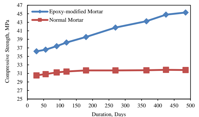
Figure 2 Strength development of epoxy-modified mortar with prolong dry-curing
