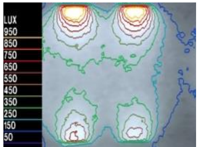
Figure 14 Spatial Illuminance distributions (North-south) orientation 14.00pm summer
