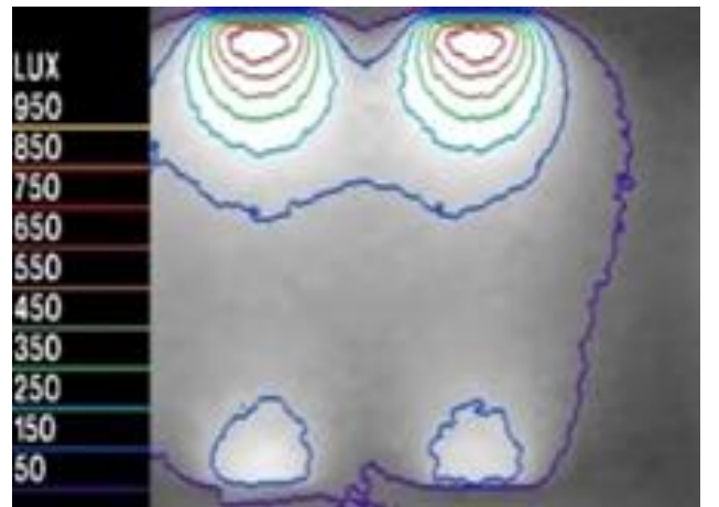
Figure 13 Spatial Illuminance distribution (North-south) orientation 9.00am winter
