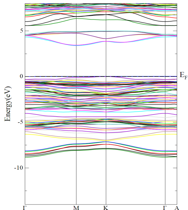
Figure 4 Band-gap structure for Mg-doped \beta -TCP material.
