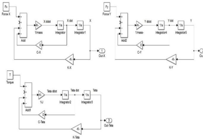
Figure 2 Simulink block diagram of the 3 DOF model of the short length drive shaft
