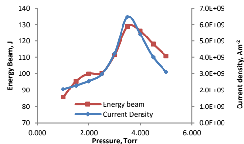
Figure 8 The correlation of current densities and energy beam with pressure for 14 kV applied voltage
