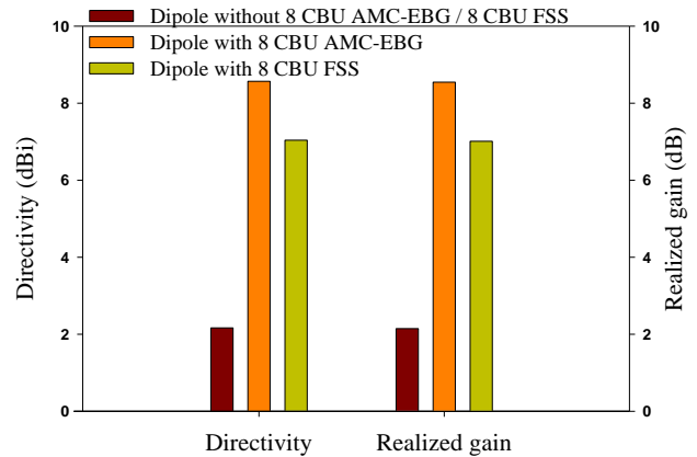
Figure 14 The comparison of performances dipole antenna with and without 8 CBU AMC-EBG and 8 CBU FSS
