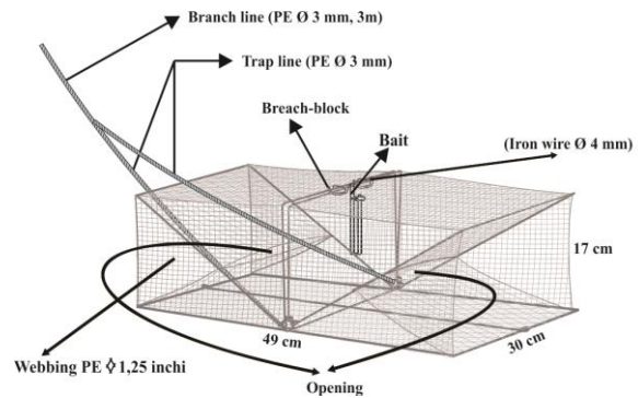
Figure 1 Construction of box fold trap
