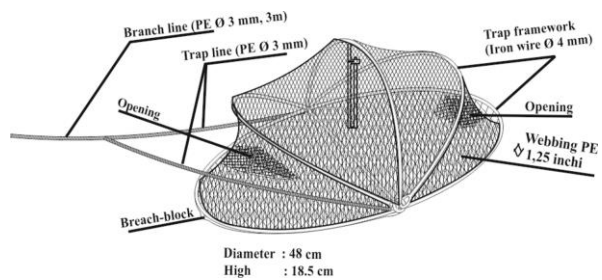
Figure 2 Construction of dome fold trap
